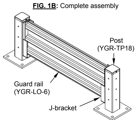
FIG. 1: YGR-LO-6 guard rail and YGR-TP-18 posts installation diagram
