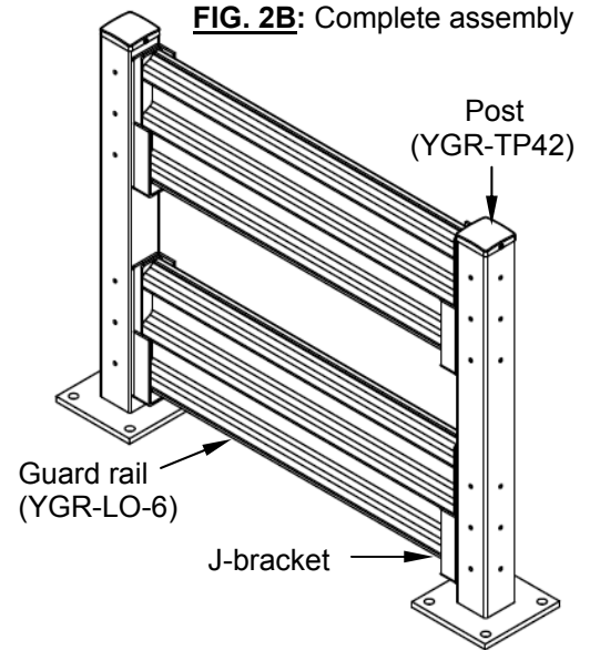
FIG. 2: YGR-LO-6 guard railing & YGR-TP42 posts installation diagram
