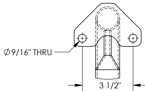
DETAIL A SCALE 1 : 4
