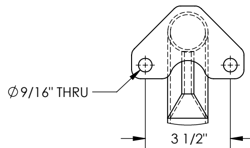
DETAIL A SCALE 1 : 4
