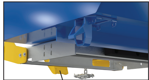
Dumping Mechanism Releases Hopper When Bumper Plate Makes Contact
