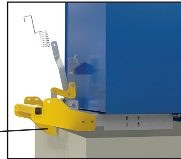
Dumping Mechanism Releases Hopper When Bumper Plate Makes Contact
