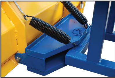
Manual Pivot and Adjustable Springs
