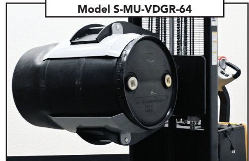
Model S-MU-VDGR-PDRM-30 Shown On Model S-MU-VDGR-64
