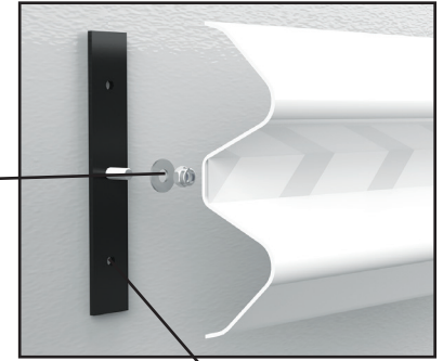
Lag Down Hardware Not Included (Bracket to Wall)
