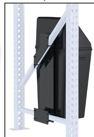
Model: WDU-RM-20-BK
